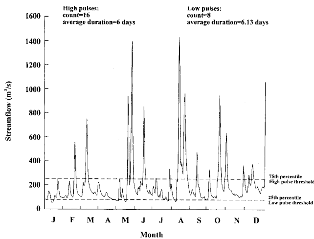
Figure 2. The computations for IHA group 4 parameters are of frequency and duration of high and low pulses. High pulses are identified as those periods during which water levels rise above the 75th percentile of all pre-impact daily flows, which is equivalent to 258 cms for the Roanoke River. Low pulses represent drops in water levels below the 25th percentile, equivalent to 97 cms.
